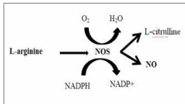
Figure 1 Nitric oxide synthesis
