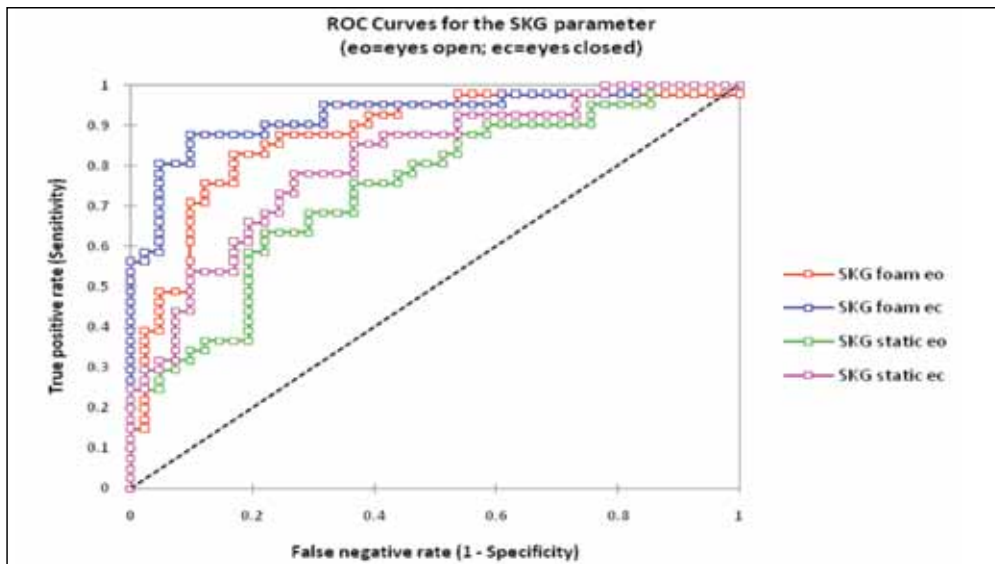
Graph 5. ROC curve evaluation for the statokinesigram parameter.
