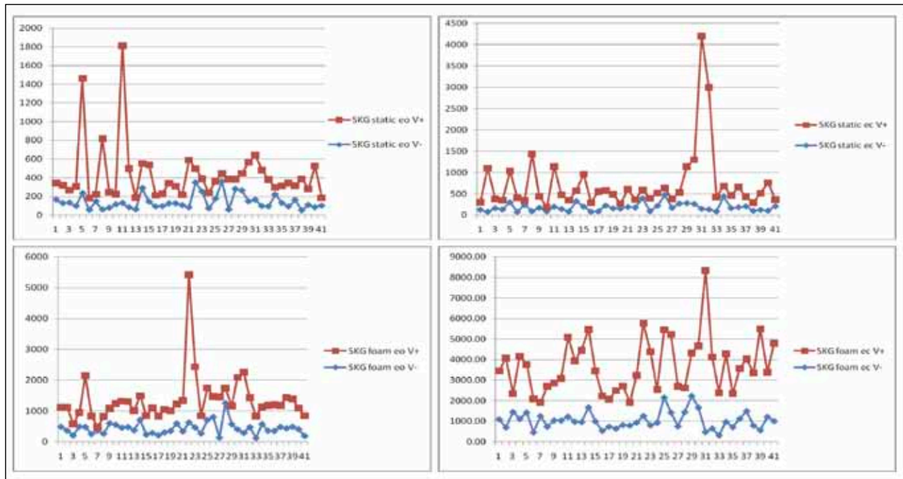
Graph 3. The graphic representation of the distribution of the statokinesigram values on static platform and foam rubber in the eyes open and eyes closed conditions (comparison between the two groups).
