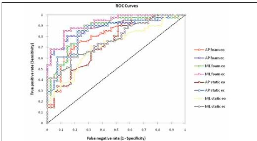
Graph 7. ROC curves representation for the maximum deviation of the centre of pressure in the AP and ML plane, on both foam and static platform (eo – eyes open, ec – eyes closed).
