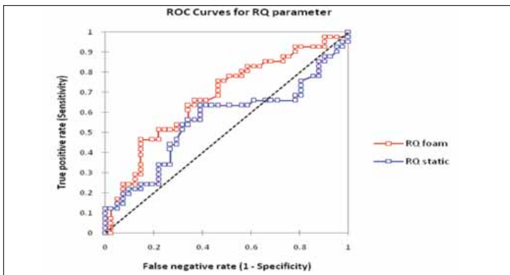
Graph 6. ROC curve representation for Romberg's quotient on both static surface and foam rubber.
