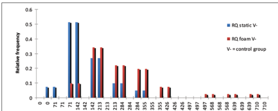
Graph 2. Representation of Romberg's quotient (RQ) values in the control group.
